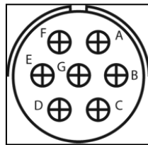
Figure 18. Input Connector View
