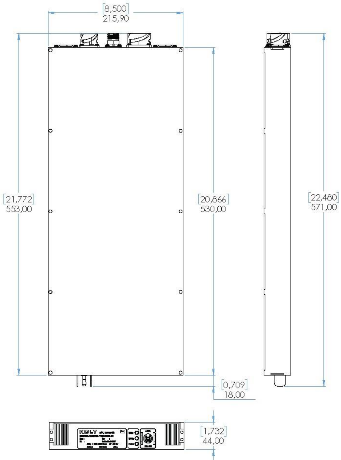
Figure 26. Mechanical Dimensions
