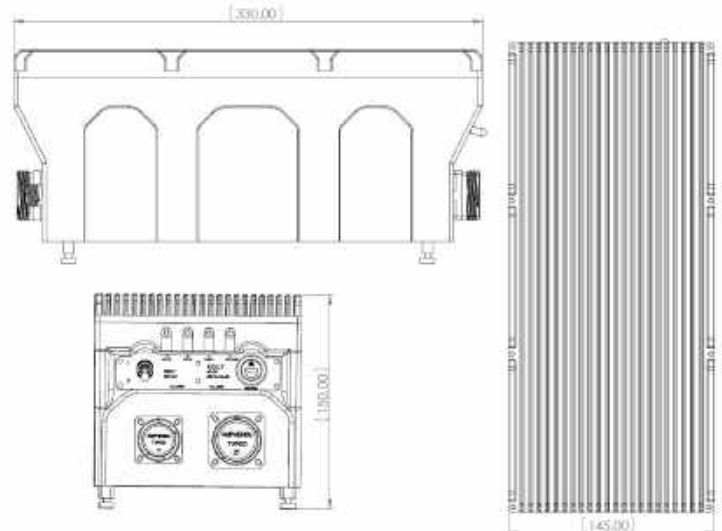
Mechanical Drawing(mm)
