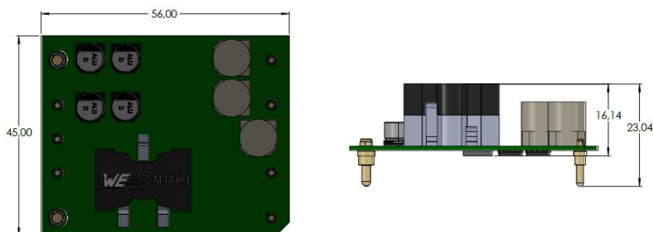
Outline Drawing(mm)
